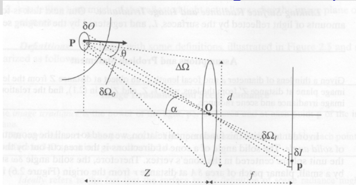
Figure 2.7 Radiometry of the image formation process.
