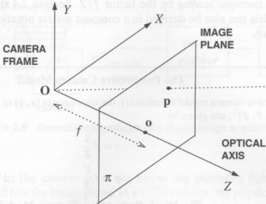
Figure 2.8 The perspective camera model.
