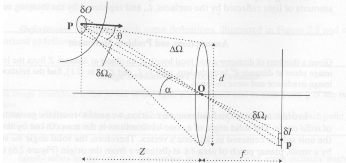
Figure 2.7 Radiometry of the image formation process.
