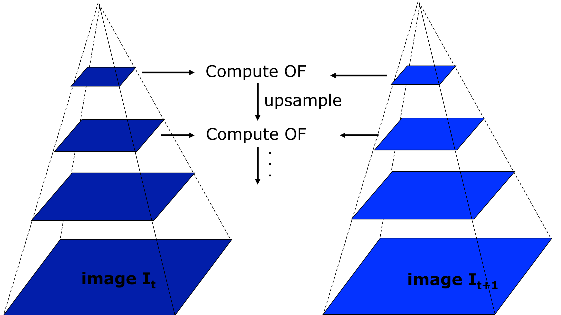
Gaussian pyramid of image I_{t+1} Motion
